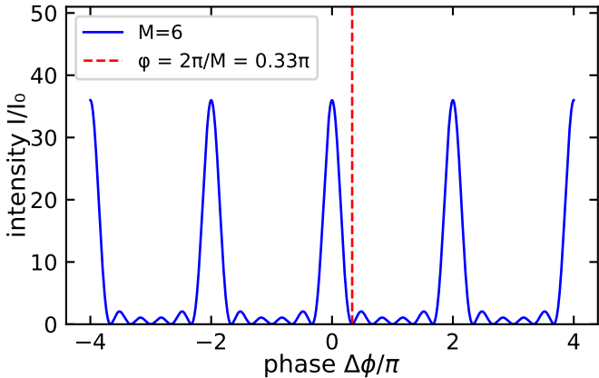
Multiple Beam Interference Pattern (M=6)
